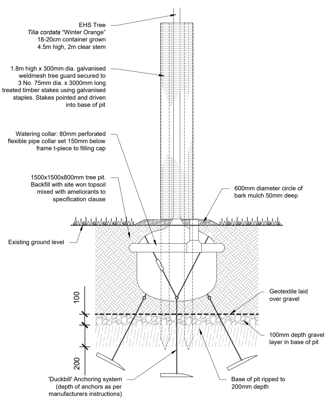
Extra Heavy Standard Planting Section 1:20
